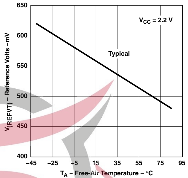
Figure 7. V_{(RefVT)} vs Temperature, V_{CC} = 2.2\text{ V}
